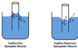
Capillary Action Mechanism for Hydrophilic and Hydrophobic Surfaces
